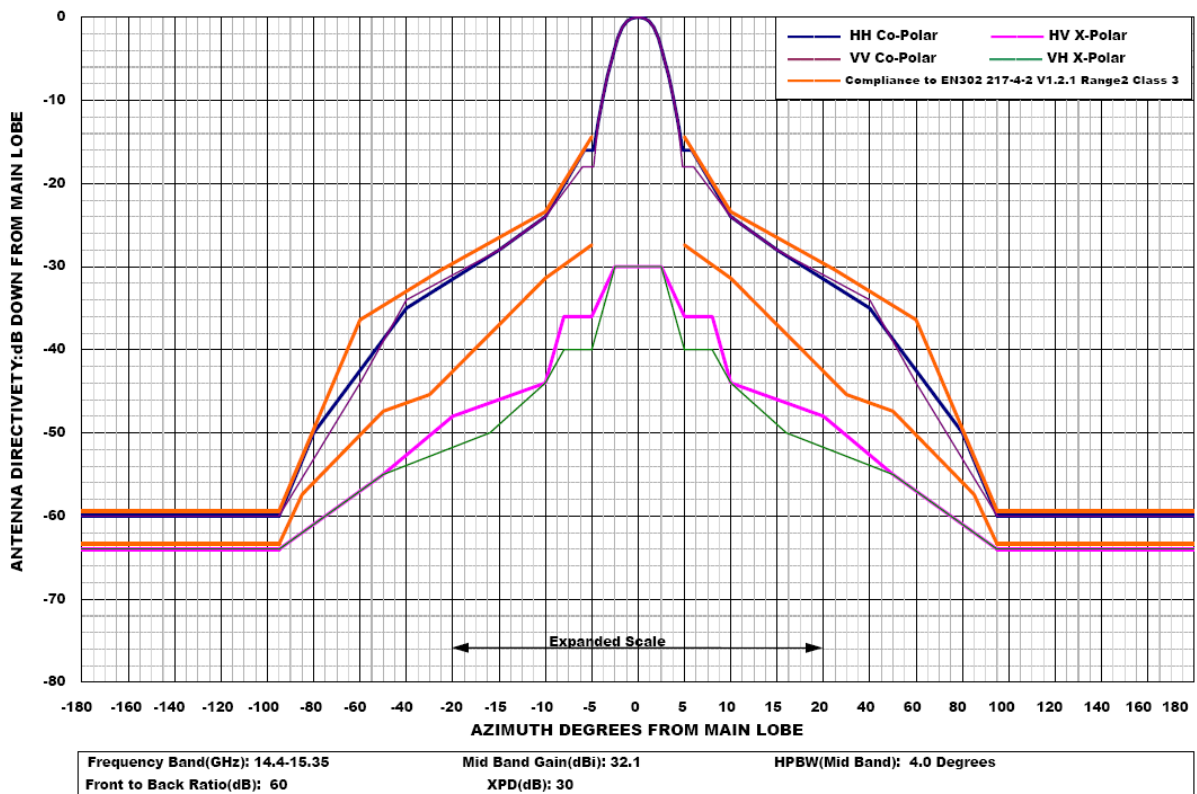
0.3m 14.4-15.35GHz RADIATION PATTERN ENVELOPE
